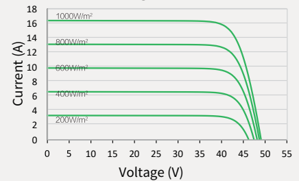
Power-Voltage (625W)
