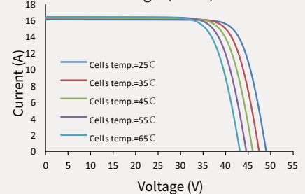
Current-Voltage (625W)
