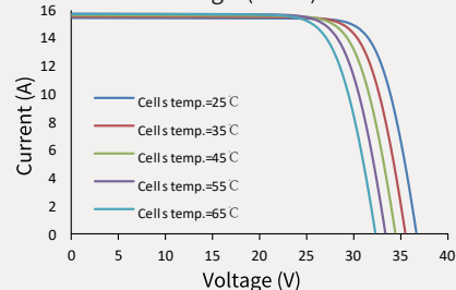
Current-Voltage (460W)
